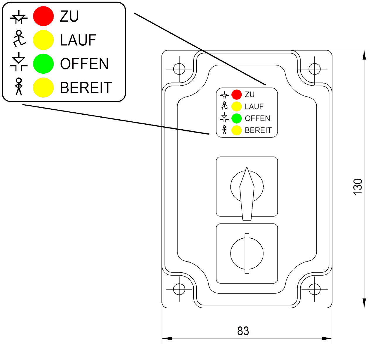
Figure 1: Switch housing with LED display
